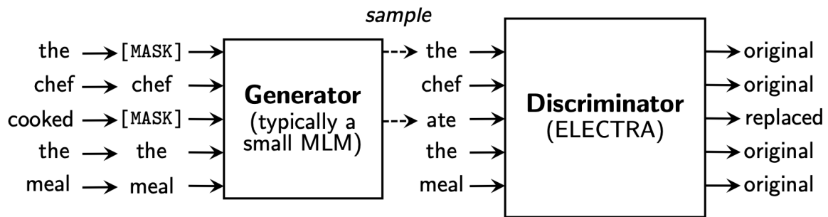
Figure 10 – Electra replaced token strategy.
